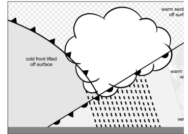
Warm front occlusion
